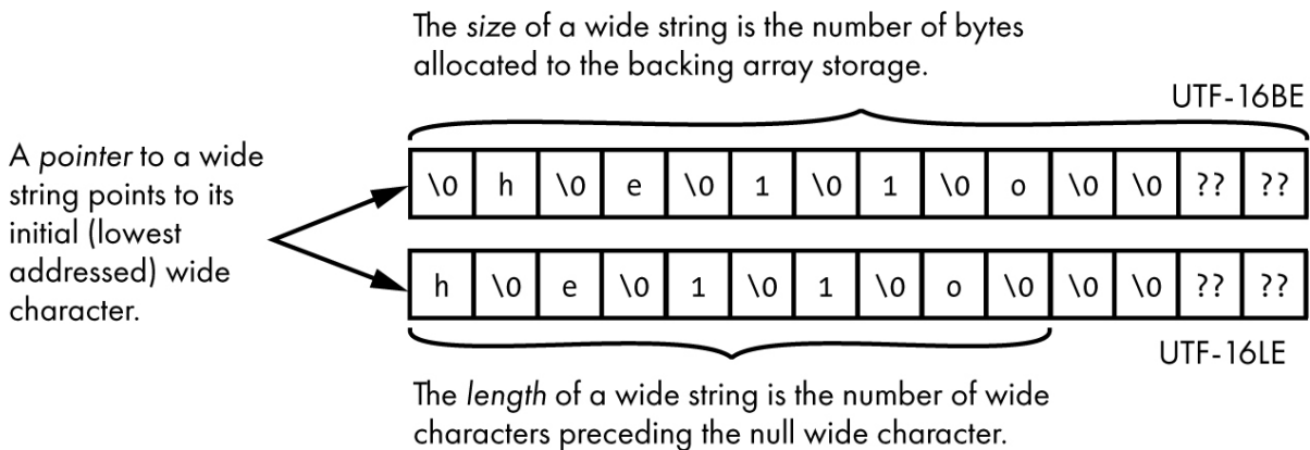
Figure 7-2: Sample UTF-16LE wide string
