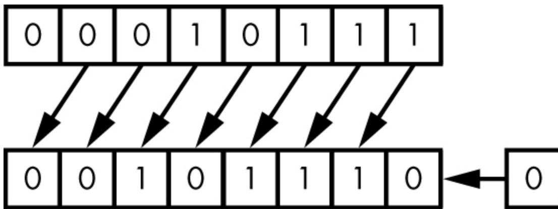
Figure 4-1: Logical left shift of 1 bit
