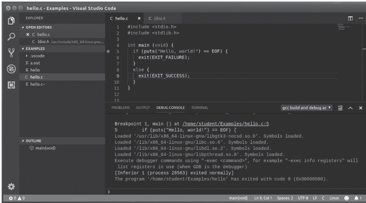
Figure 1-2: Visual Studio Code running on Ubuntu
