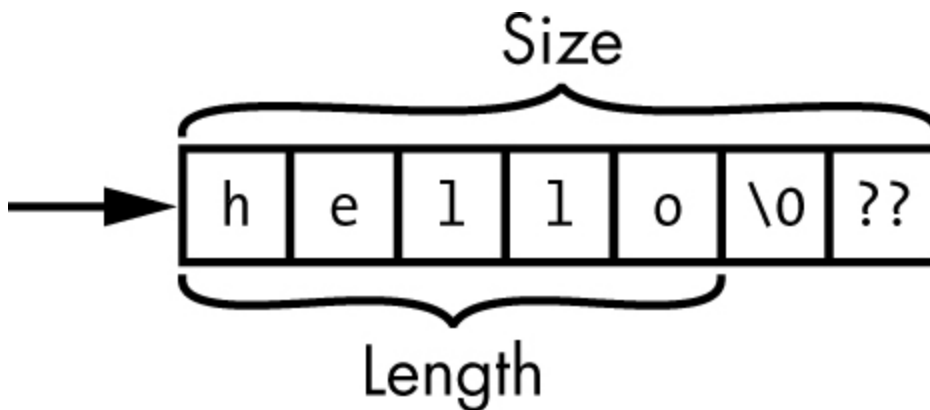
Figure 7-1: Sample narrow string
