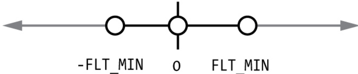
Figure 3-3: Domain of subnormal numbers
