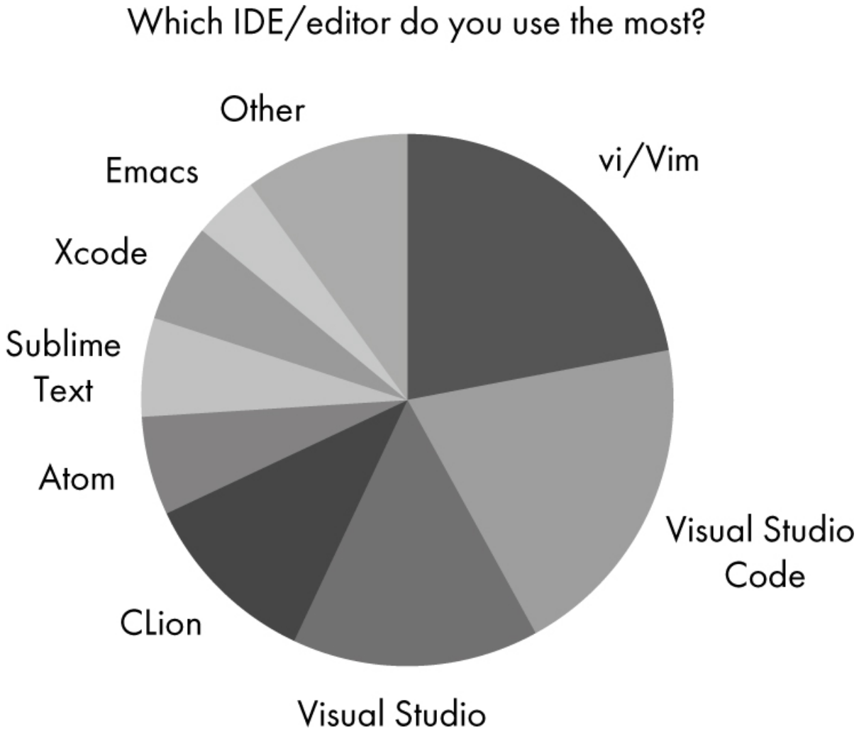
Figure 1-1: IDE/editor use
