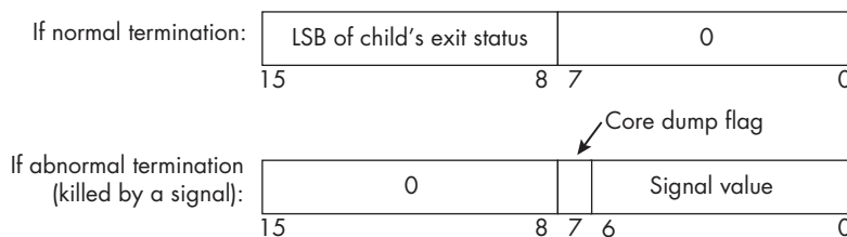
Figure 11-5: A traditional arrangement of bits of the status available from the call wait(&status)
