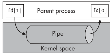
Figure 13-2: The pipe immediately after creation by the parent process
