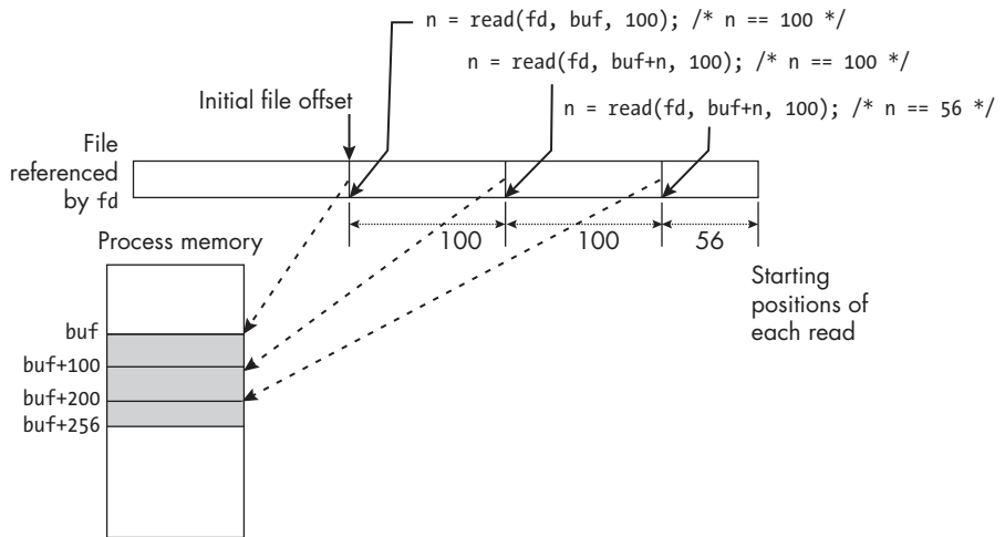
Figure 4-3: Three successive reads with the third returning fewer bytes than requested
