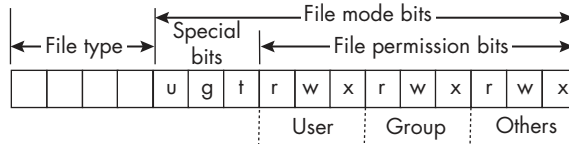
Figure 6-9: The file mode bits in the st_mode member
