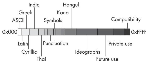
Figure B-1: Unicode layout
