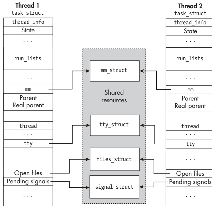
Figure 15-1: A schematic representation of how the process descriptors of two threads that are part of the same process facilitate sharing of memory, open files, and other shared data of the parent process
