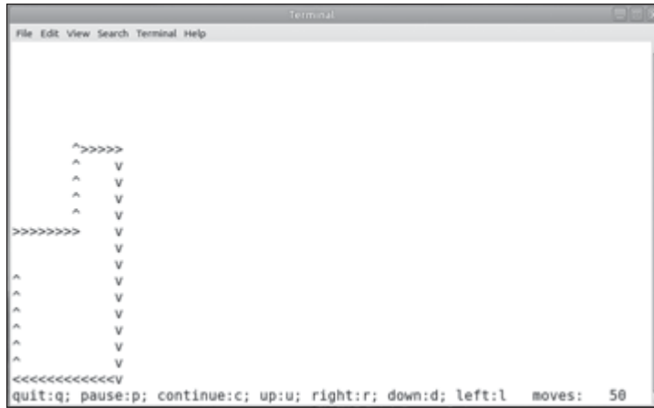
Figure 19-3: A screenshot of the running sprite_curses.c program
