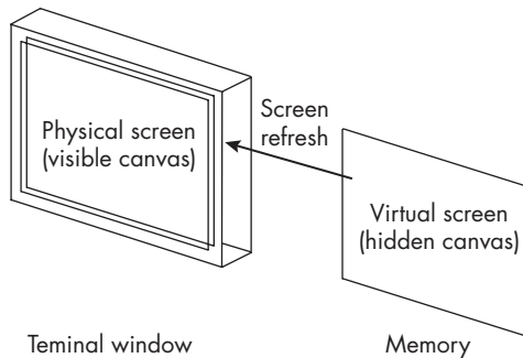
Figure 19-2: Screen refreshing in which the contents of a hidden canvas are applied to the visible canvas on the screen
