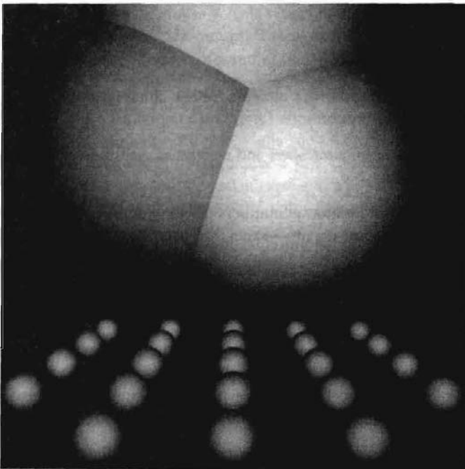
Figure 9.7: Ray-traced image.
