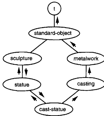
Figure 11.3: Class hierarchy.
