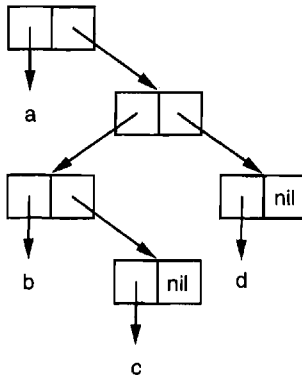
Figure 3.8: Binary tree.
