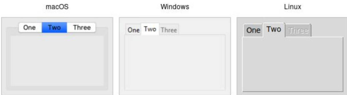
Notebook widgets.
