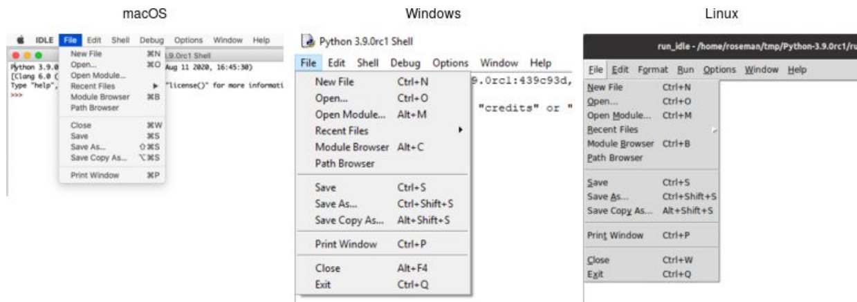
Menubars.
