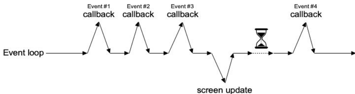
Execution timeline for well-behaved event loop.
