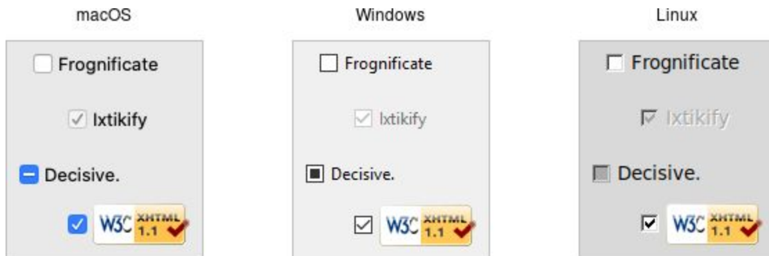
Checkbutton widgets.
