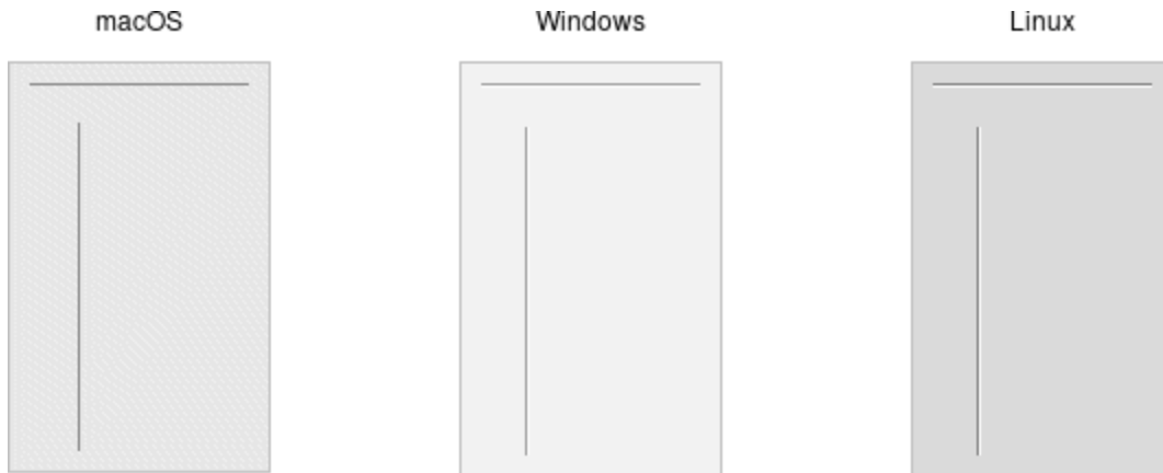
Separator widgets.
