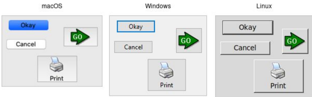
Button widgets.
