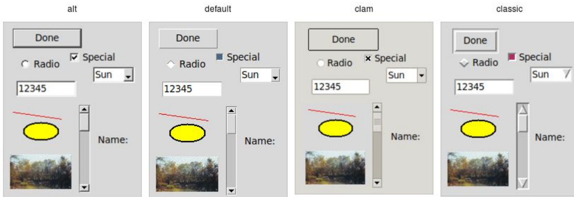
Built-in themes.
