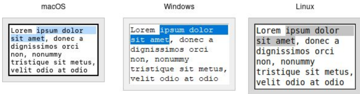
Text widgets.
