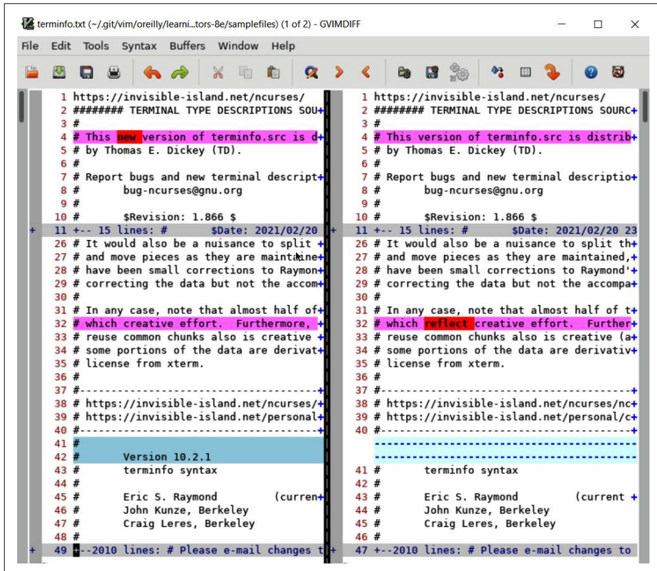
Figure 13-7. vimdiffe results (WSL Ubuntu gvimdiff, color scheme: zellner)
